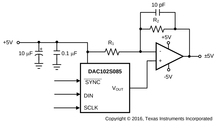
Figure 37. Bipolar Operation
