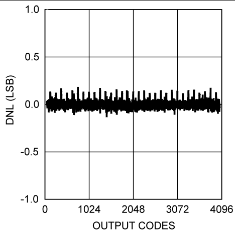
Figure 5. DNL at V_A = 3\text{ V}
