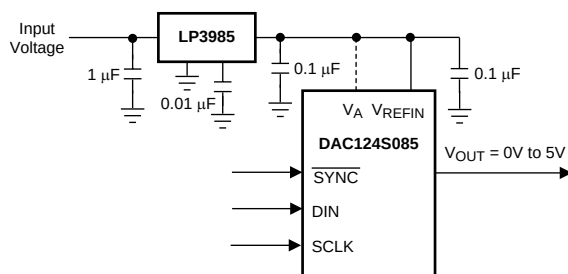
Figure 39. LP3985 Regulator
