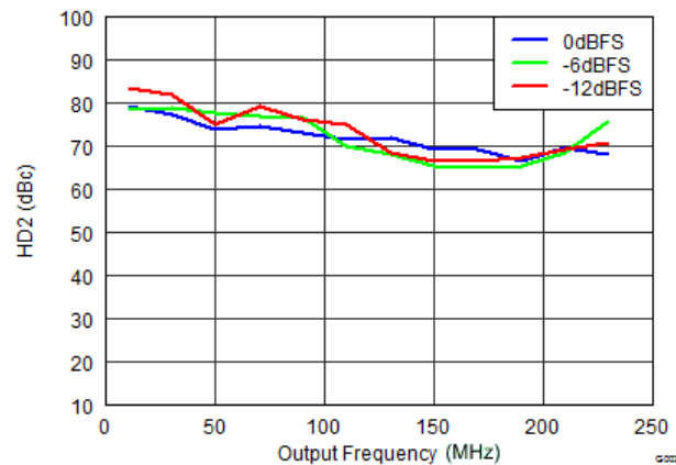
Figure 8. Second-Order Harmonic Distortion vs Output Frequency Over Input Scale
