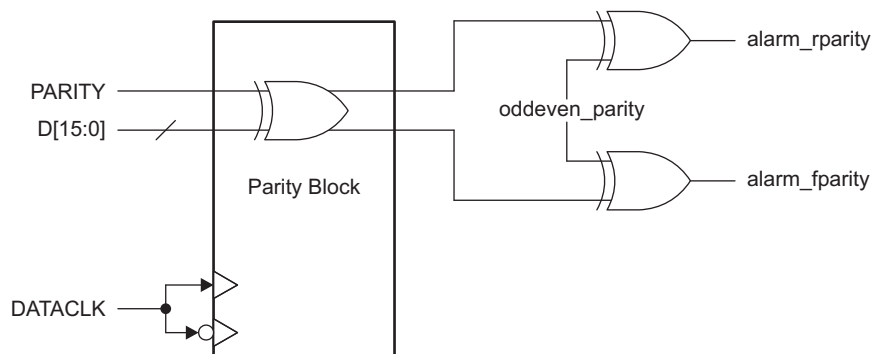
图 77. DAC3484 Word-by-Word Parity Check
