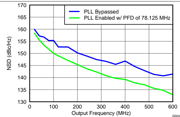
图 24. NSD vs Output Frequency Over Clocking Options
