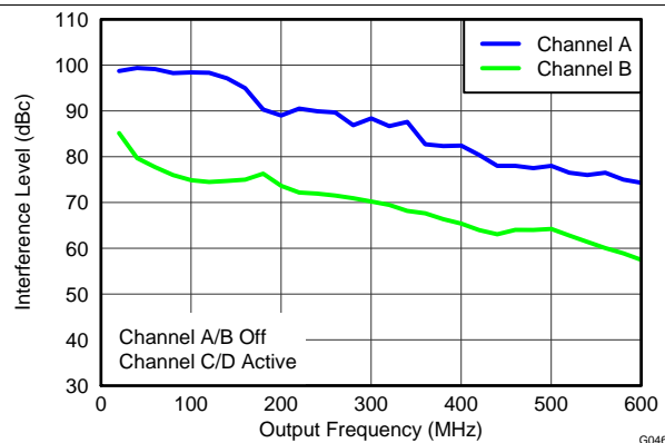
图 46. Channel Isolation vs Output Frequency
