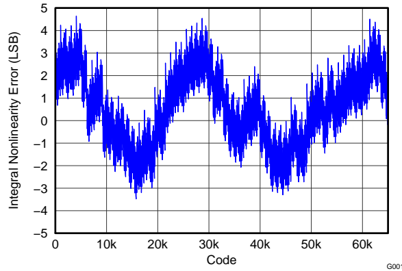
图 1. Integral Nonlinearity
