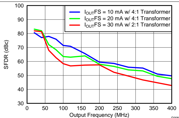
图 8. SFDR vs Output Frequency Over I_{OUTFS}
