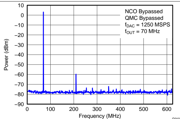
图 10. Single Tone Spectral Plot
