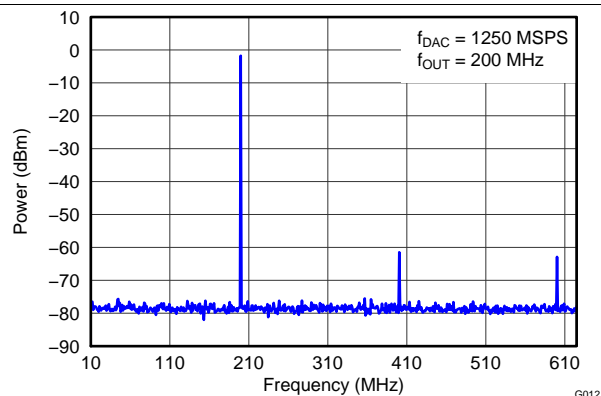
图 12. Single Tone Spectral Plot
