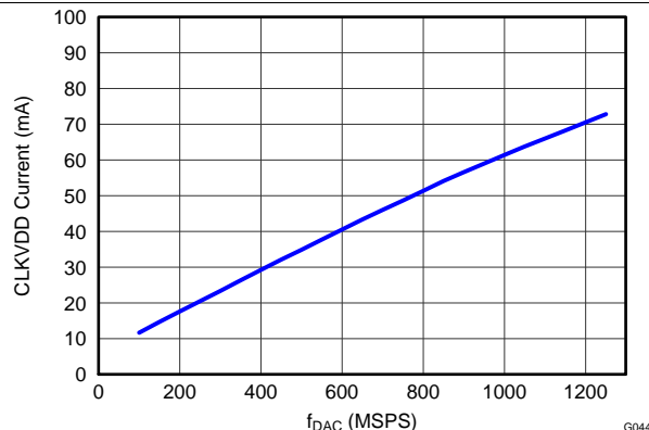
图 44. CLKVDD Current vs f_{DAC}
