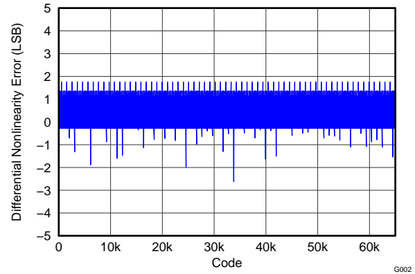
图 2. Differential Nonlinearity
