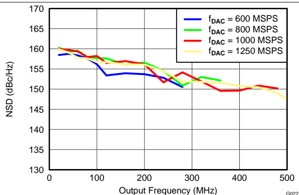
图 22. NSD vs Output Frequency Over f_{DAC}
