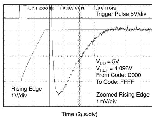
Figure 13. Full-Scale Settling Time: 5-V Rising Edge
