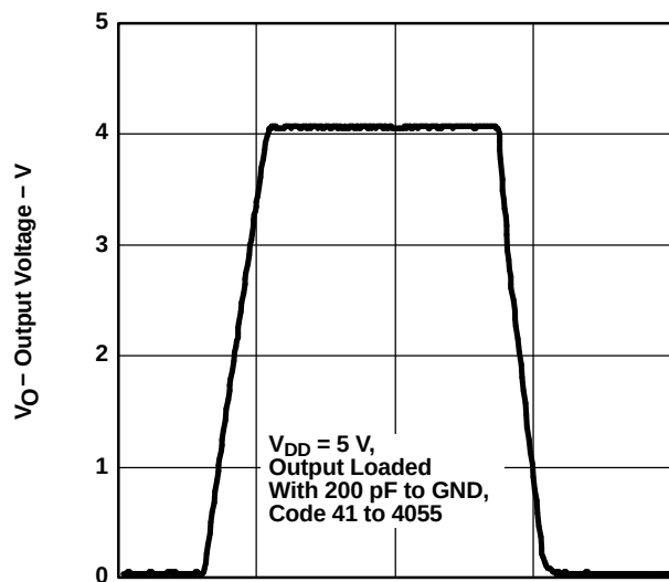
LARGE-SIGNAL SETTLING TIME - 5 V
