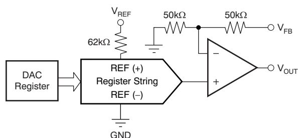
Figure 27. DAC8551-Q1 Architecture
