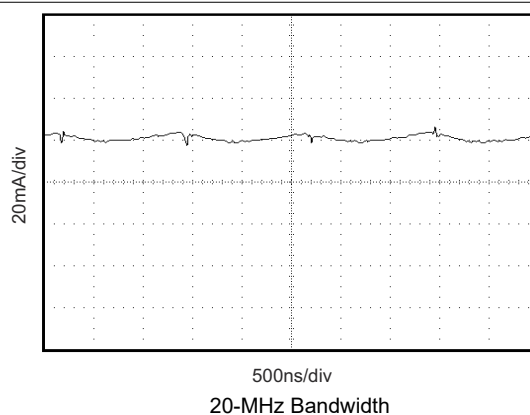
图 7-16. Input Current Reflected Ripple
