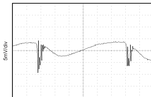
图 7-16. Input Current Reflected Ripple
