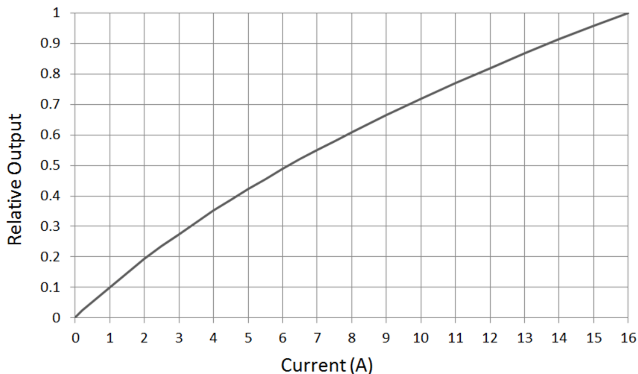
图 8-2. Luminance vs Current
