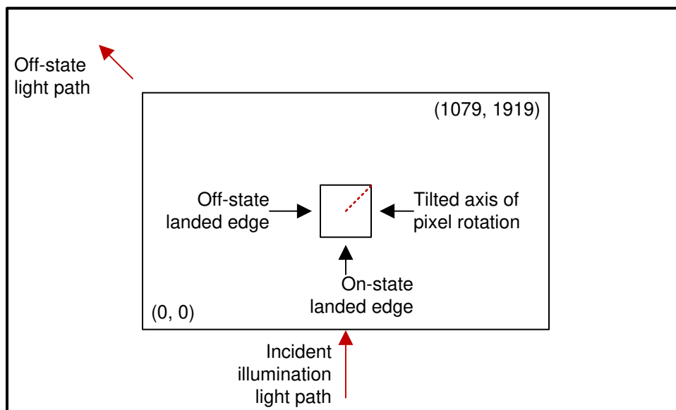
图 6-17. Landed Pixel Orientation and Tilt
