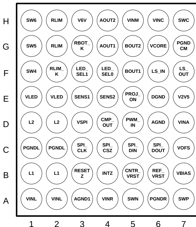
Pin Functions
