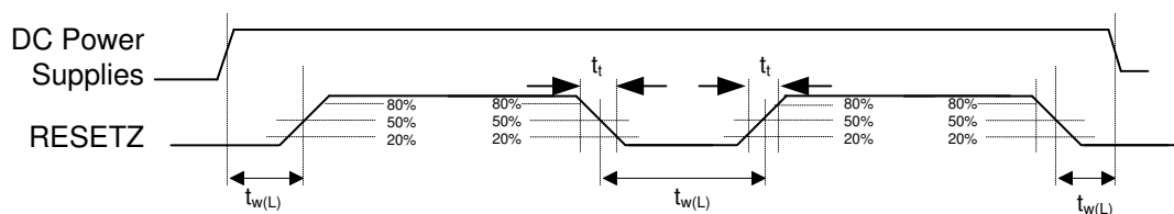
Figure 4. Power-Up and Power-Down RESETZ Timing
