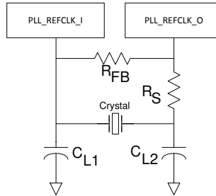
图 8-12. Discrete Components Required When Using Crystal
