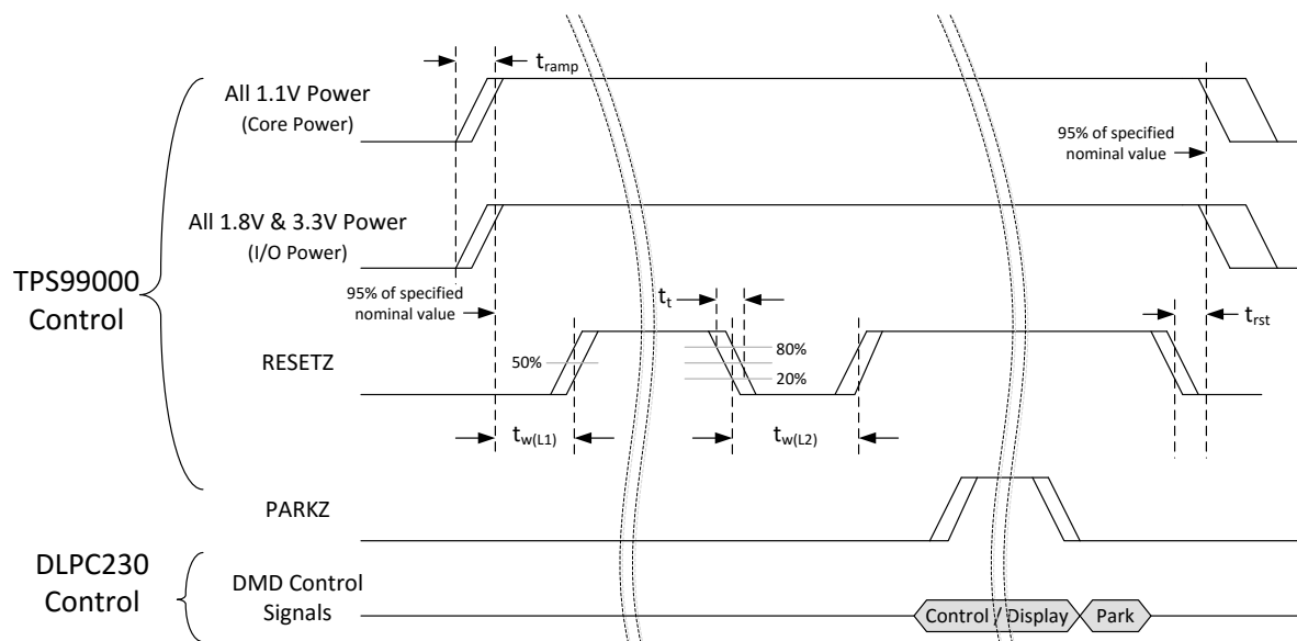
图 5-2. Power Supply and RESETZ Timing
