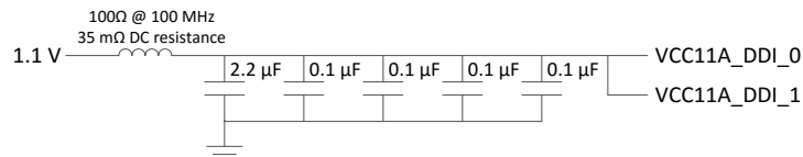
图 8-4. VCC11A_DDI Recommended Filter
