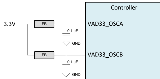
图 9-11. Crystal Power Supply Filtering
