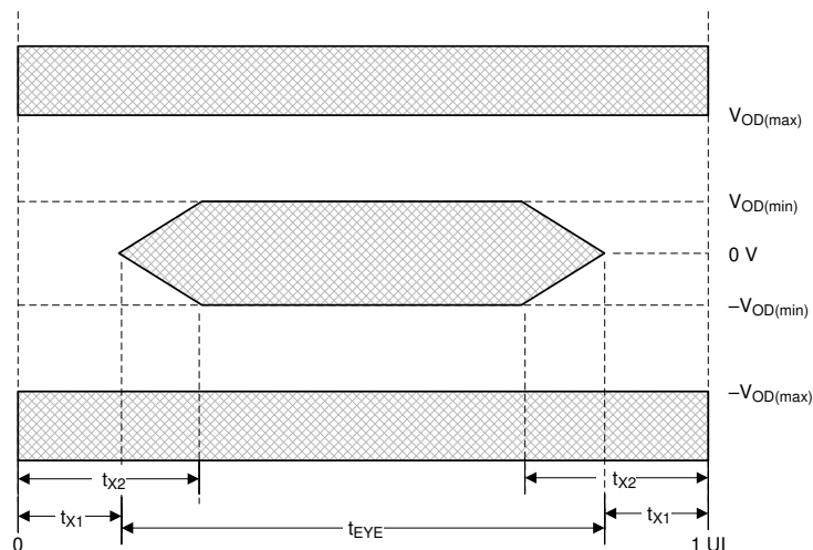
图 6-11. HSSI Eye Characteristics
