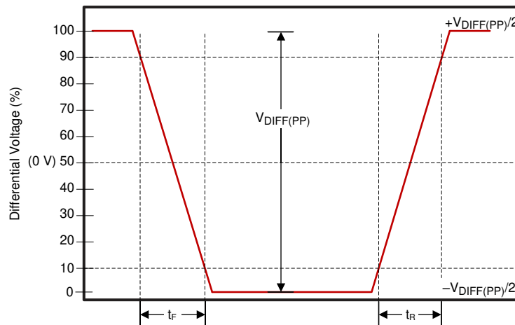
图 6-12. DMD Low-Speed Differential Timing Parameters
