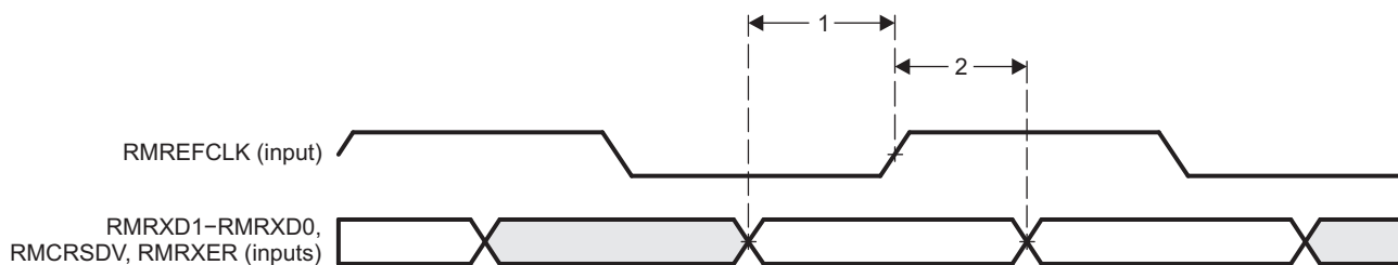
Figure 8-15. EMAC Receive Interface Timing RMII Operation
