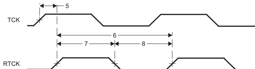
Figure 8-8. JTAG With RTCK Timing
