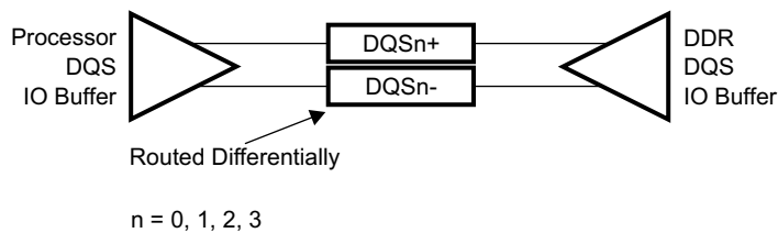
Figure 8-77. DQS Topology
