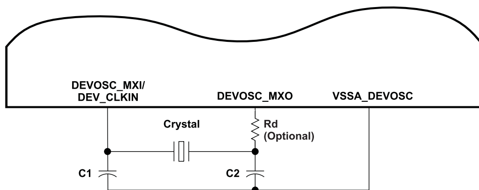
Figure 7-8. Device Oscillator
