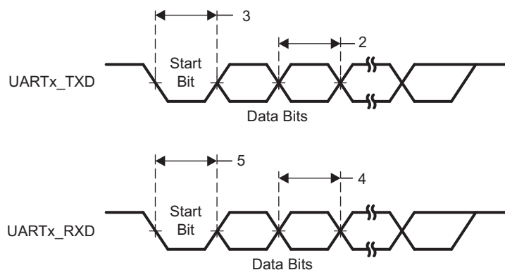
Figure 8-98. UART Timing
