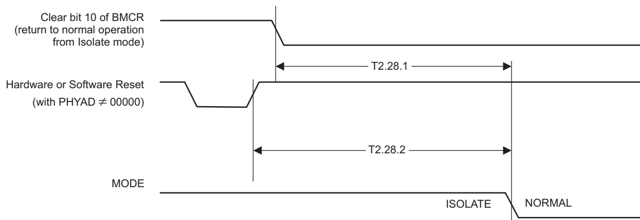
图 4-29. Isolation Timing
