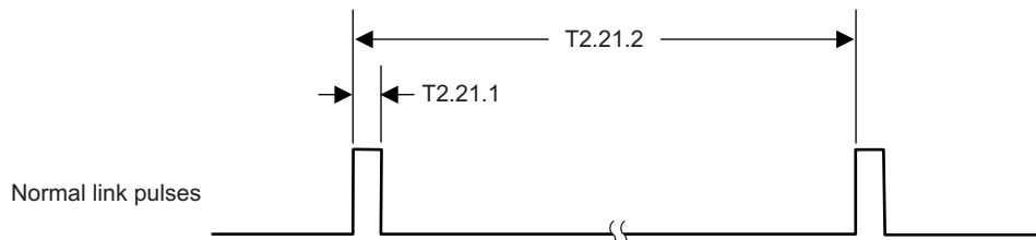
图 4-22. 10BASE-T Normal Link Pulse Timing
