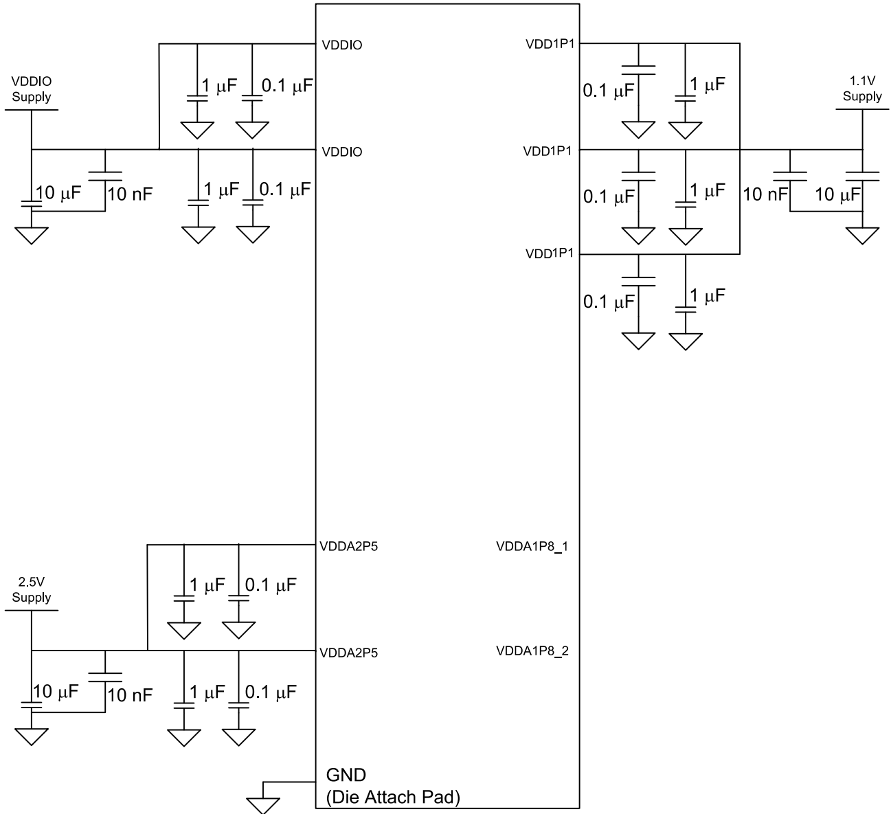
图 8-8. Two-Supply Configuration
