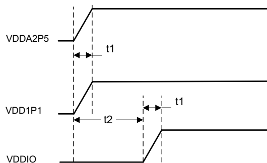
图 8-9. Two-Supply Sequence Diagram
