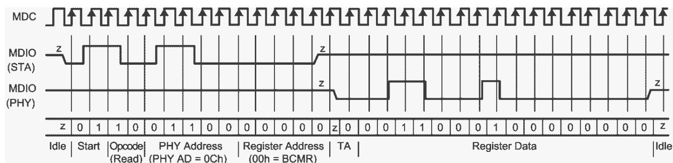
图 7-13. Typical MDC/MDIO Read Operation
