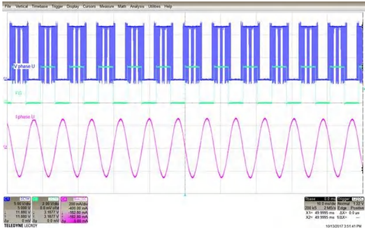
图 7-1. 180° Sensorless-Control Scheme
