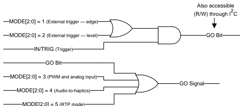
Figure 19. GO-Signal Logic
