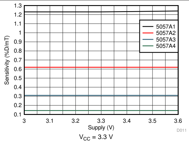
图 2. Sensitivity vs Supply Voltage
