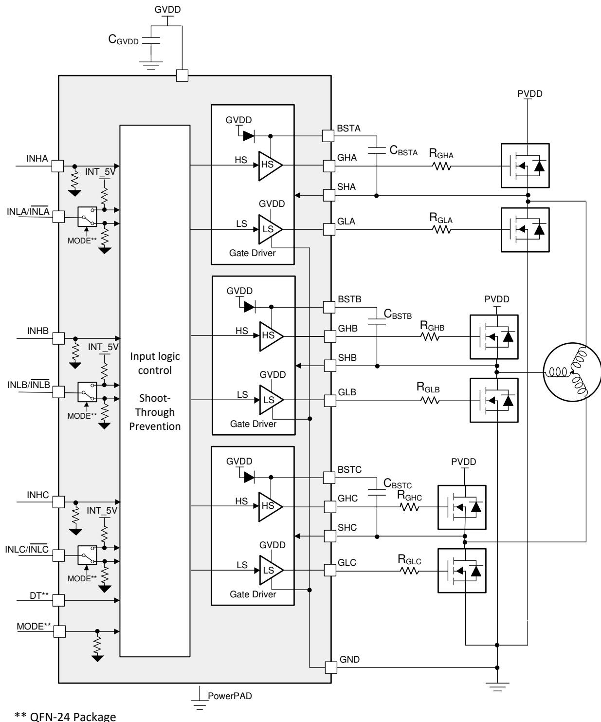
图 8-1. Block Diagram for DRV8300D
