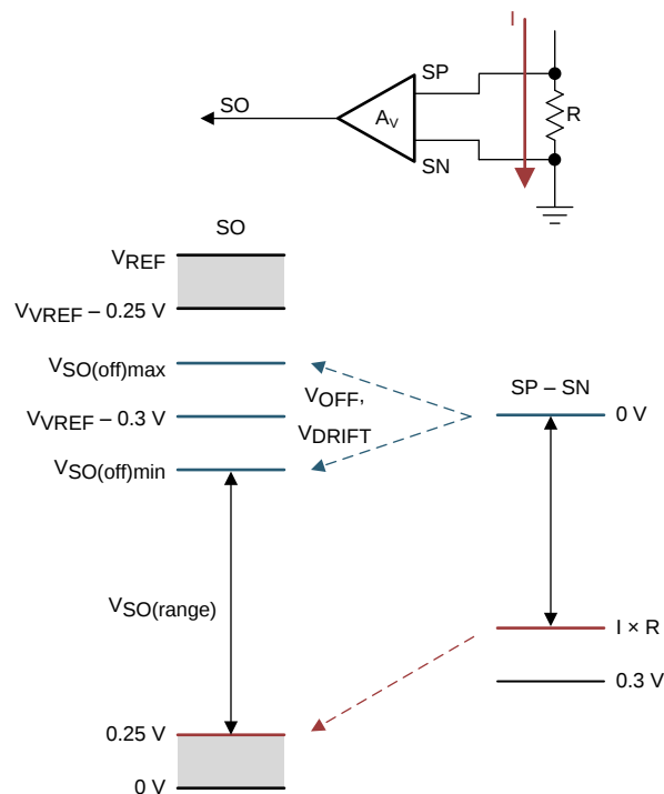
图 35. Unidirectional Current-Sense Regions
