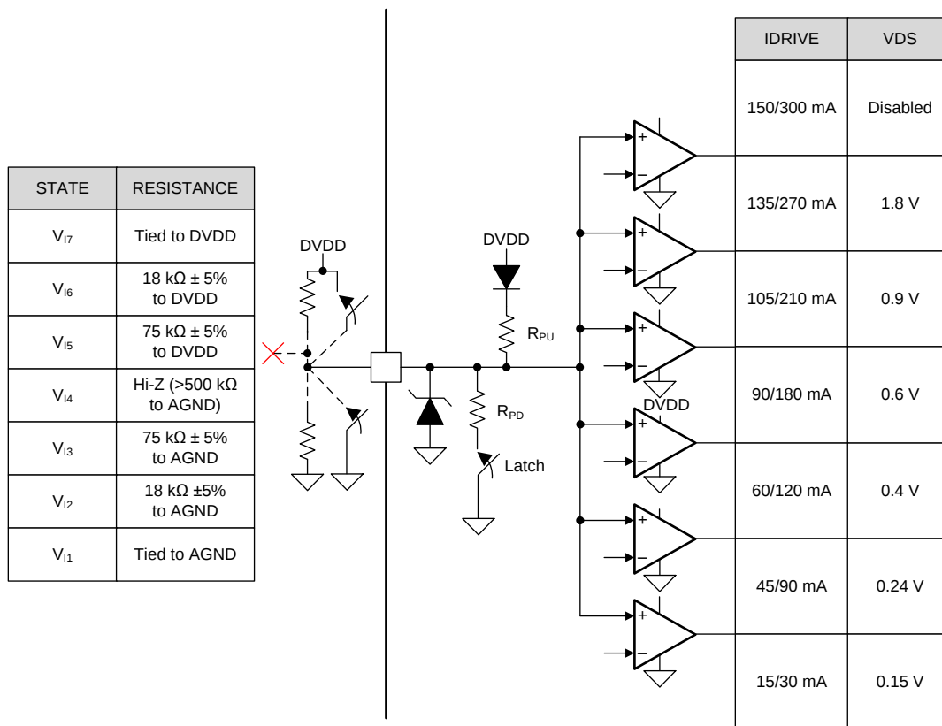
图 28. Seven-Level Input Pin Structure (IDRIIVE and VDS)
