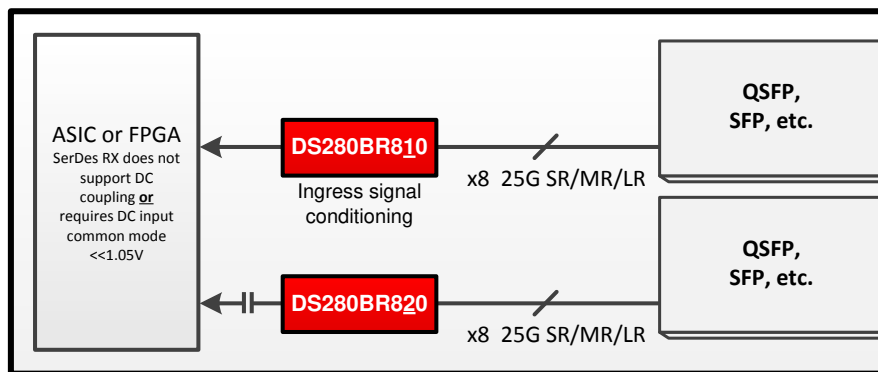
图 13. DS280BR820 or DS280BR810 Recommended for Front-port Ingress
