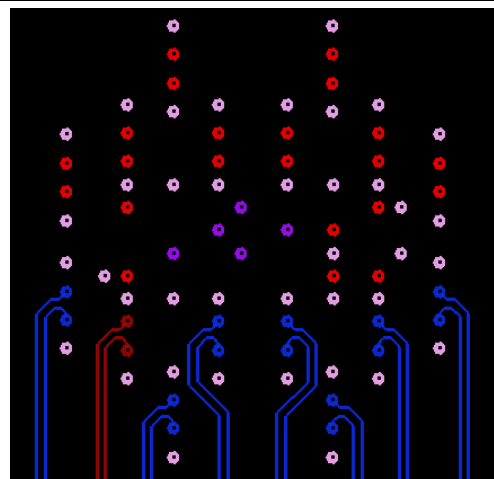
图 32. Stripline Example, Internal Signal Layer 1
