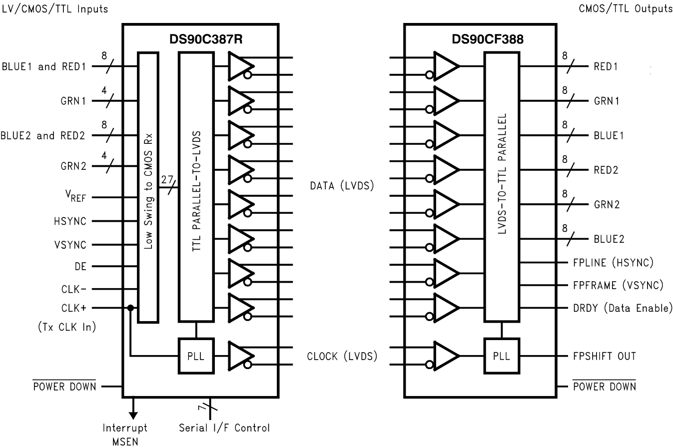
Figure 1. DS90C387R
