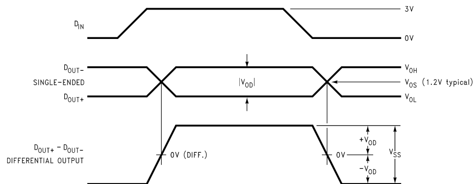
Figure 8. Driver Output Levels
