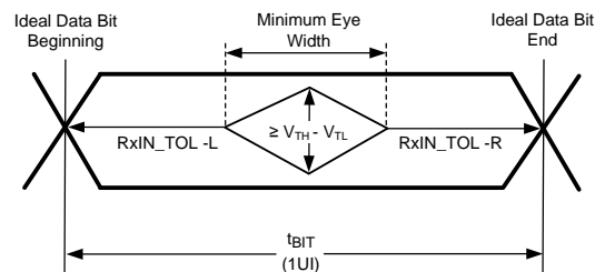
Figure 18. CMLOUT Eye Opening
