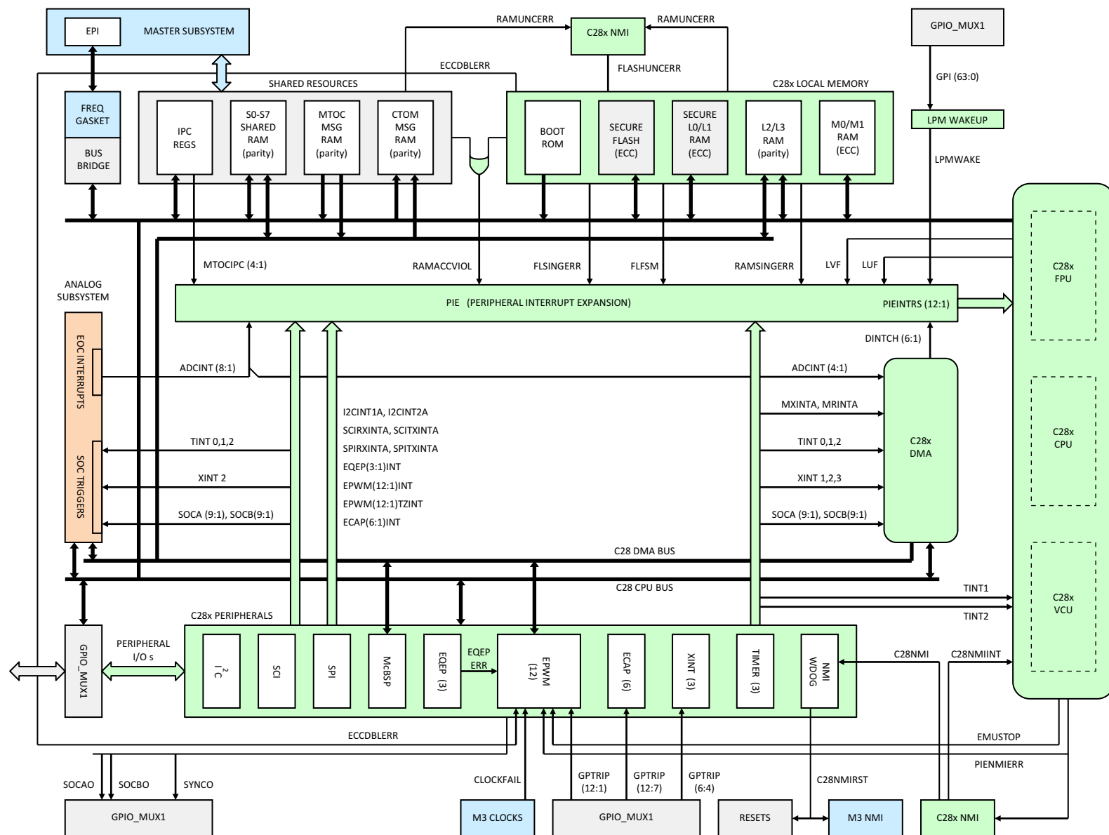
Figure 6-2. Control Subsystem
