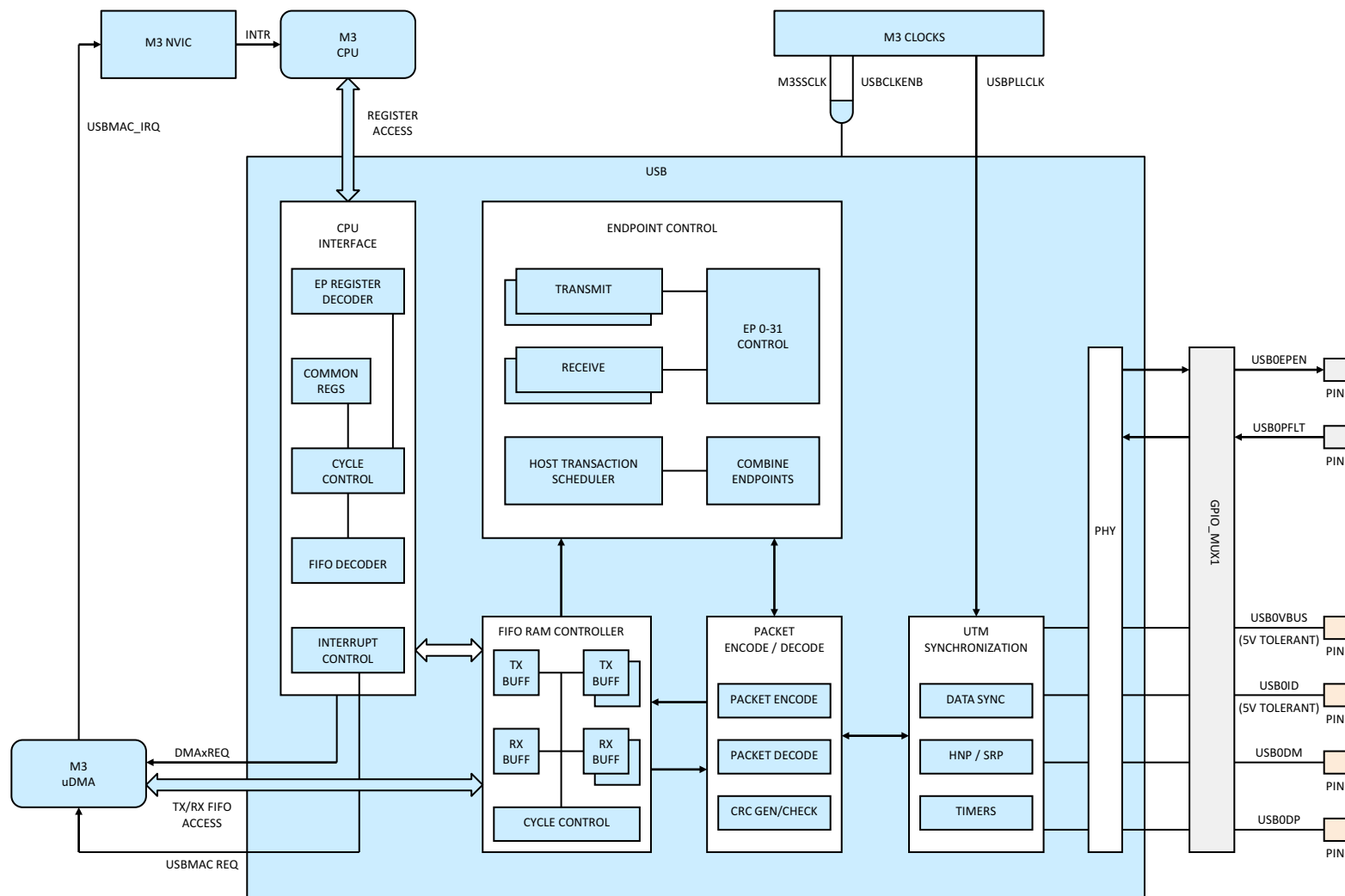
Figure 5-35. USB
