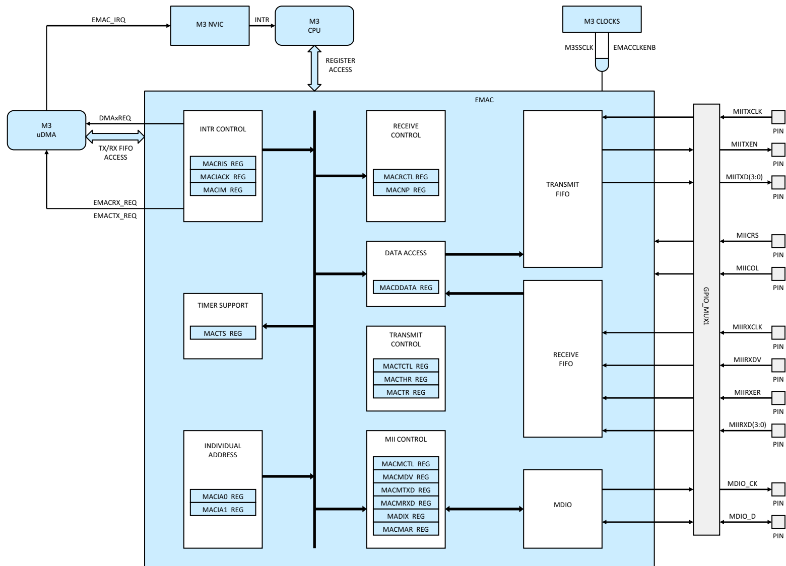
Figure 5-36. EMAC
