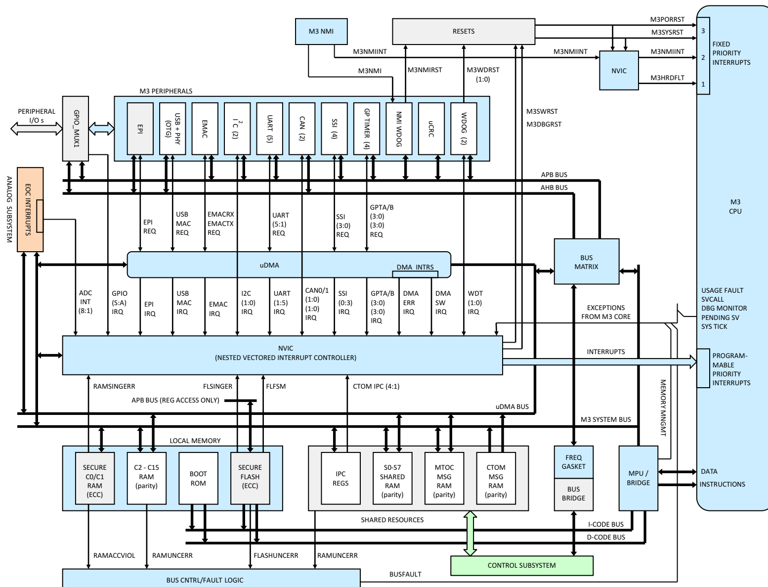
Figure 6-1. Master Subsystem
