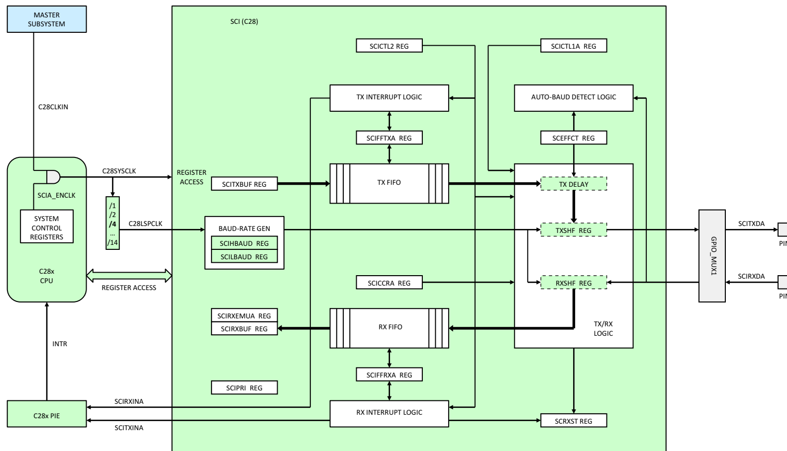
Figure 5-50. SCI (C28x)
