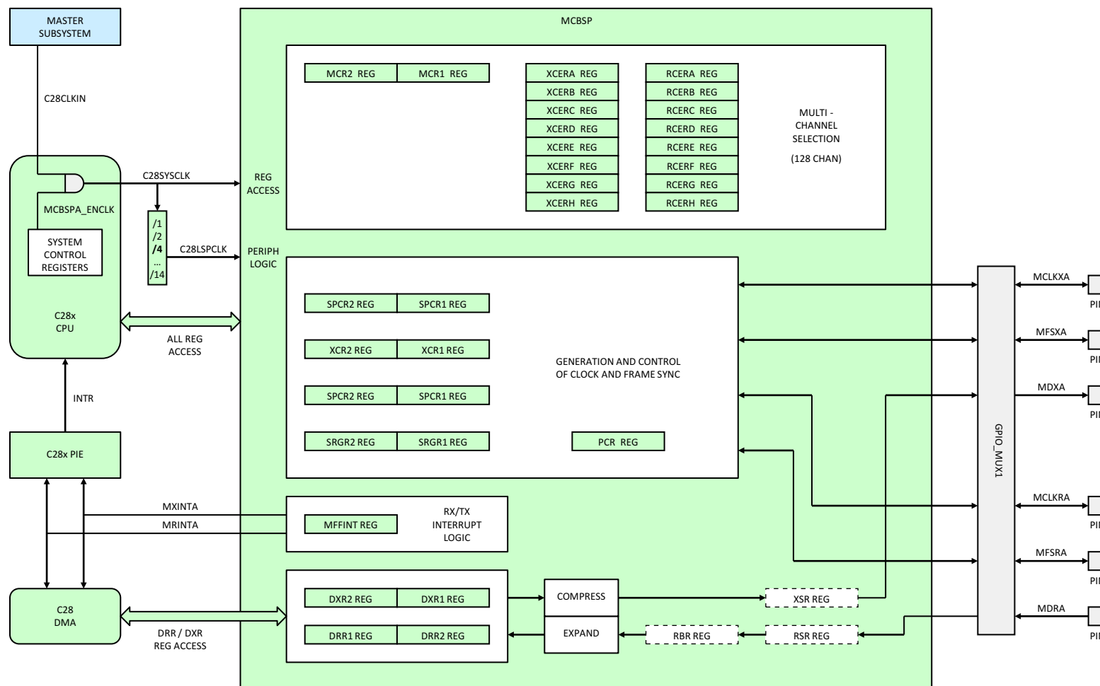
Figure 5-56. McBSP (C28x)
