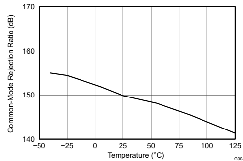
图 6-4. Shunt Input Common-Mode Rejection Ratio vs. Temperature
