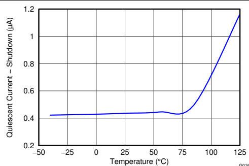
图 6-16. Shutdown I_Q vs. Temperature
