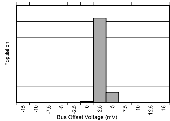
图 6-8. Bus Input Offset Voltage Production Distribution
