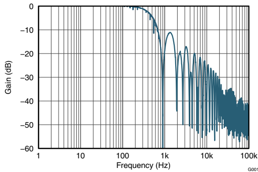
图 6-1. Frequency Response
