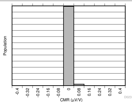
图 5-14. Input Common-Mode Rejection Distribution
