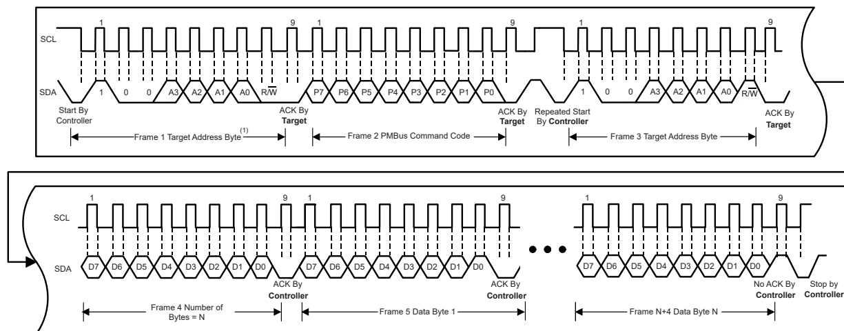
图 6-6. Timing Diagram for Block Read Format
