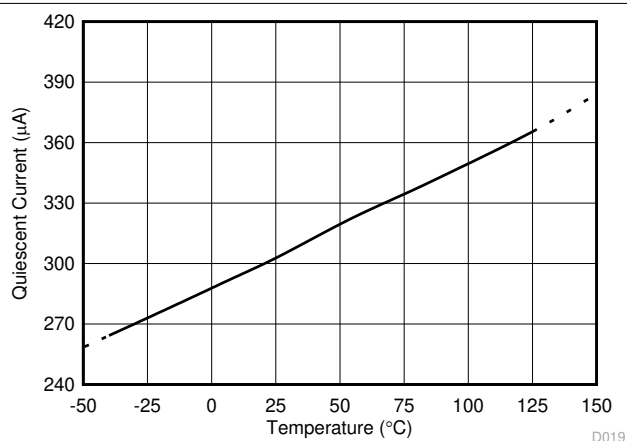
图 5-19. Active I_Q vs Temperature
