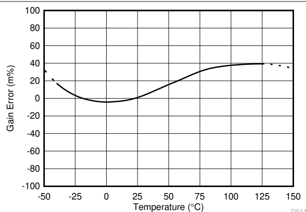
图 5-11. Bus Input Gain Error vs Temperature
