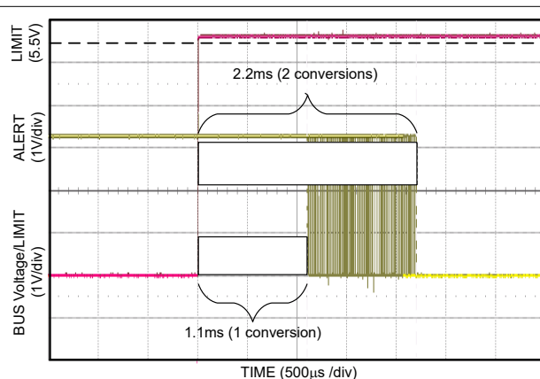
图 7-3. Alert Response ( t_{CT} = 1.1ms )
