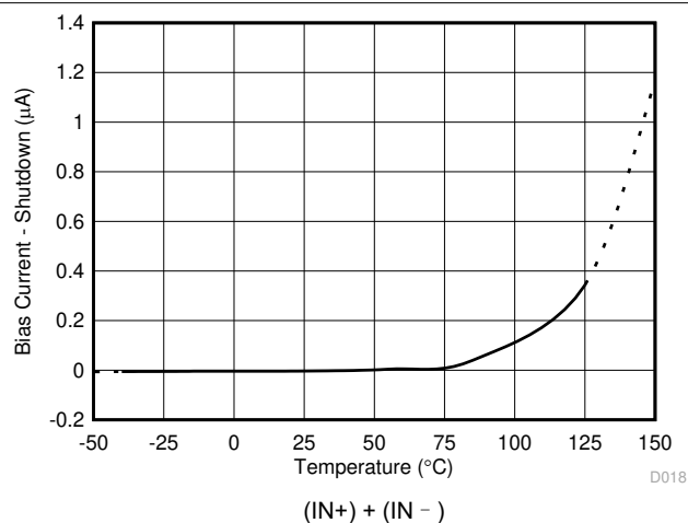
图 5-18. Input Bias Shutdown Current vs Temperature
