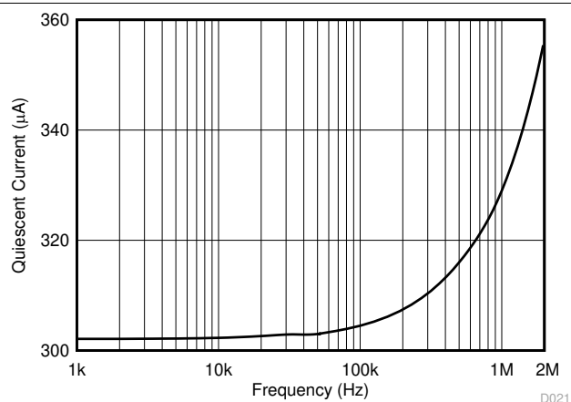
图 5-21. Active I_Q vs SCL Frequency
