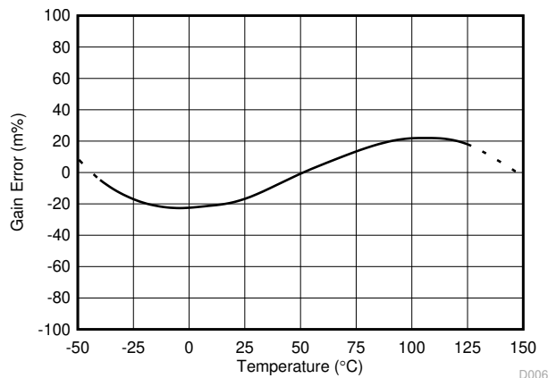
图 5-6. Shunt Input Gain Error vs Temperature
