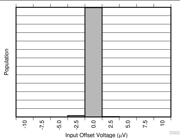
图 5-2. Shunt Input Offset Voltage Production Distribution
