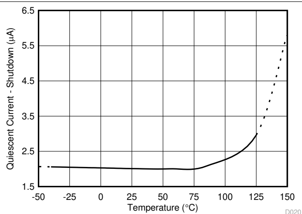
图 5-20. Shutdown I_Q vs Temperature
