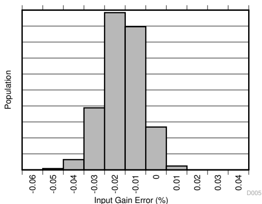
图 5-5. Shunt Input Gain Error Production Distribution
