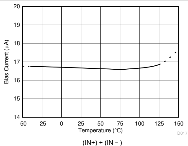
图 5-17. Input Bias Current vs Temperature
