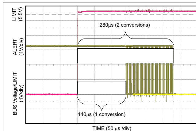
图 7-2. Alert Response ( t_{CT} = 140\mu s )
