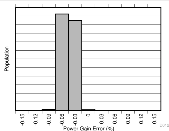
图 5-12. Power Gain Error Production Distribution
