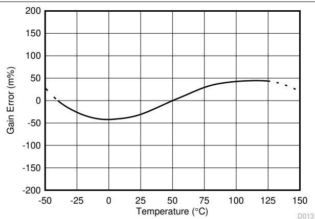
图 5-13. Power Gain Error vs Temperature
