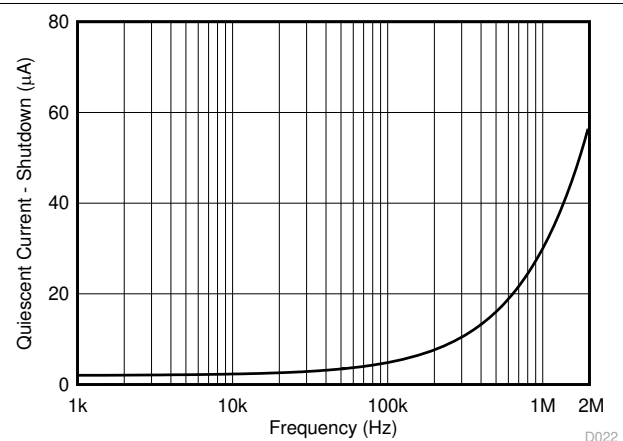
图 5-22. Shutdown I_Q vs SCL Frequency
