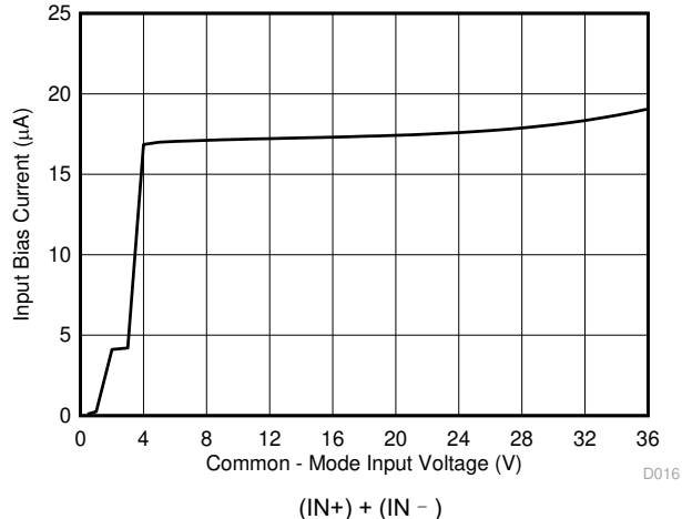
图 5-16. Input Bias Current vs Common-Mode Voltage
