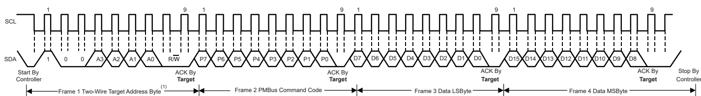
图 6-4. Timing Diagram for Write Word Format
