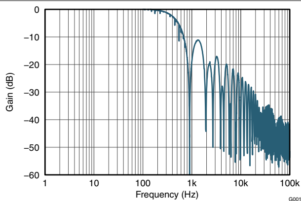
图 5-1. Frequency Response
