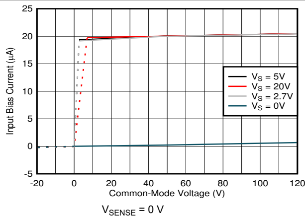
图 6-5. Input Bias Current vs Common-Mode Voltage
