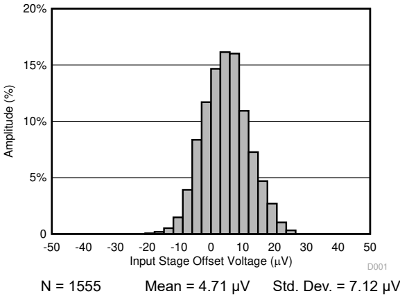
图 7-1. Typical Distribution of Input Stage Offset Voltage
