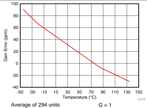
图 30. Gain Error vs Temperature, G = 1
