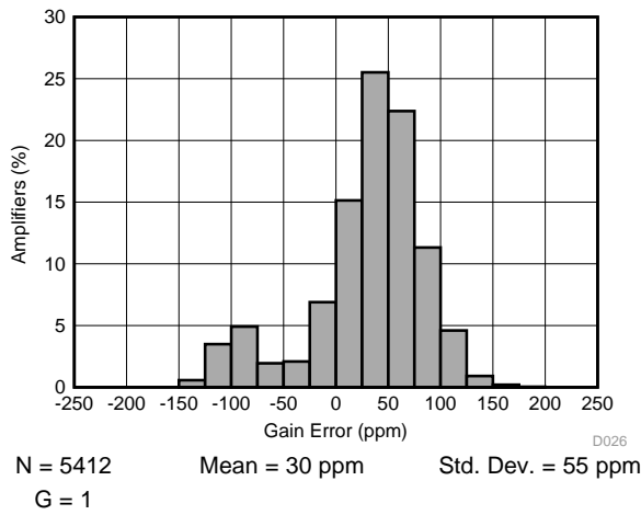
图 27. Typical Distribution of Gain Error, G = 1
