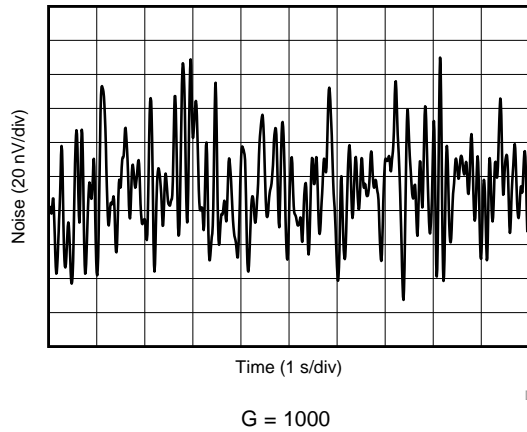
图 25. 0.1-Hz to 10-Hz RTI Voltage Noise, G = 1000
