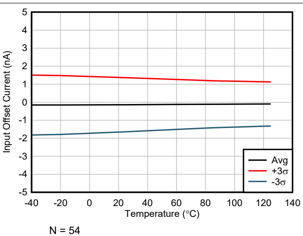
图 7-16. Input Offset Current vs Temperature
