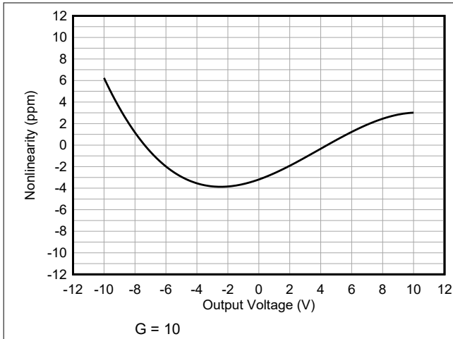
图 7-35. Gain Nonlinearity, G = 10
