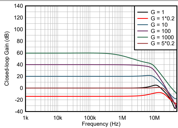
图 7-24. Gain vs Frequency
