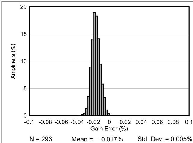
图 7-11. Typical Gain Error Distribution at G = 0.2 V/V
