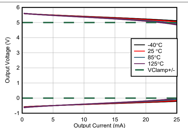
图 7-38. Positive Output Voltage Swing vs Output Current
