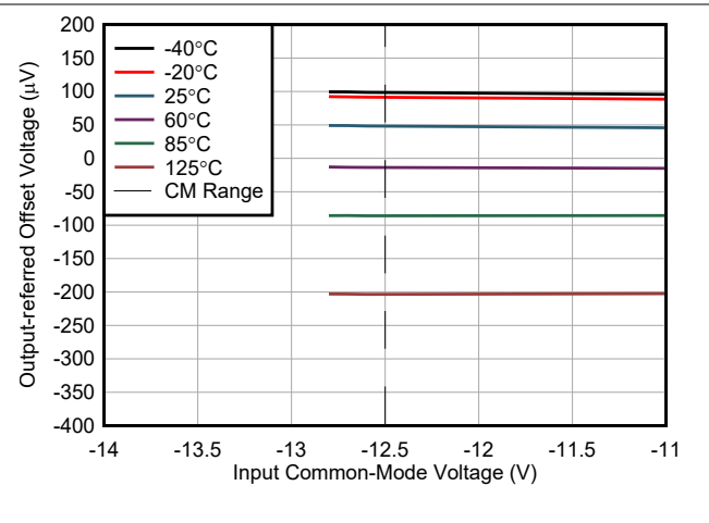
图 7-36. Offset Voltage vs Negative Common-Mode Voltage
