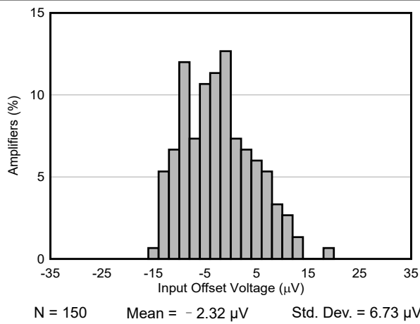
图 7-1. Typical Distribution of Input Stage Offset Voltage
