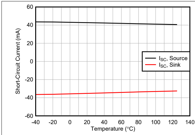
图 7-41. Short Circuit Current vs Temperature
