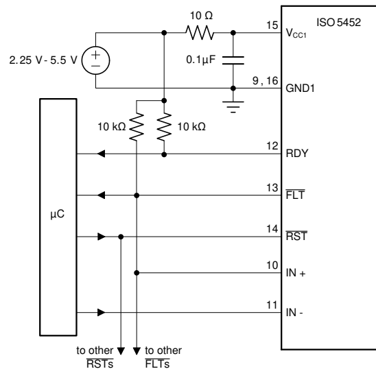
图 10-6. Global Shutdown With Inverting Input Configuration
