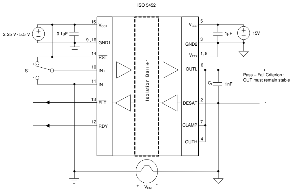
图 8-4. Common-Mode Transient Immunity Test Circuit
