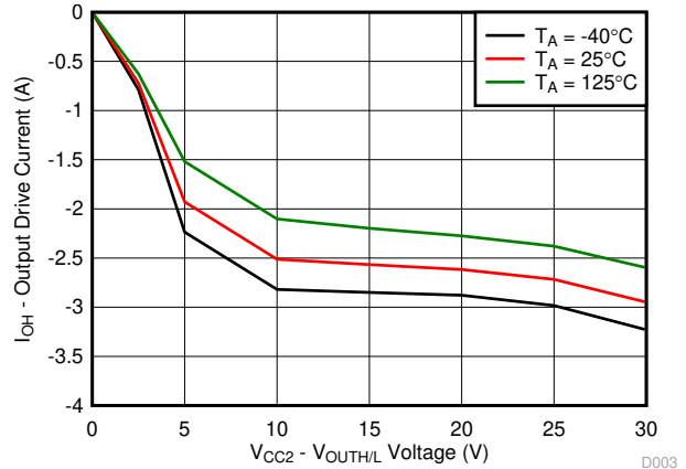
图 7-5. Output High Drive Current vs Output Voltage
