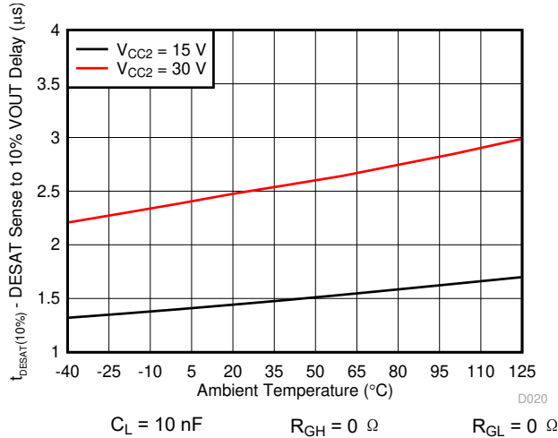
图 7-33. DESAT Sense to V_{OUT/IL} 10% Delay vs Temperature
