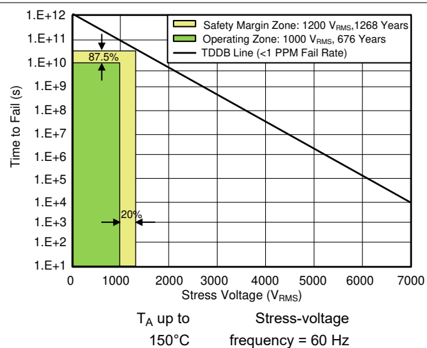
图 7-1. Reinforced Isolation Capacitor Lifetime Projection
