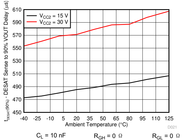
图 7-34. DESAT Sense to V_{OUT/IL} 90% Delay vs Temperature
