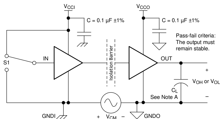
图 11. Common-Mode Transient Immunity Test Circuit
