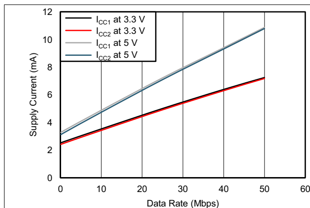
Figure 1. ISO7142 Supply Current for All Channels vs Data Rate
