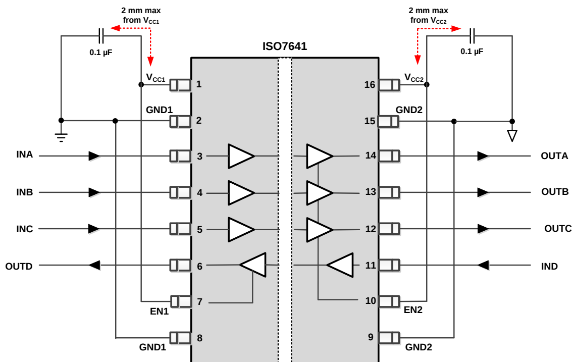
图 18. Typical ISO7641FM Circuit Hookup
