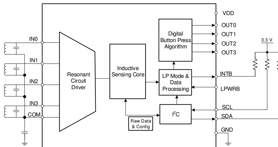
图 7-1. Block Diagram of LDC3114
