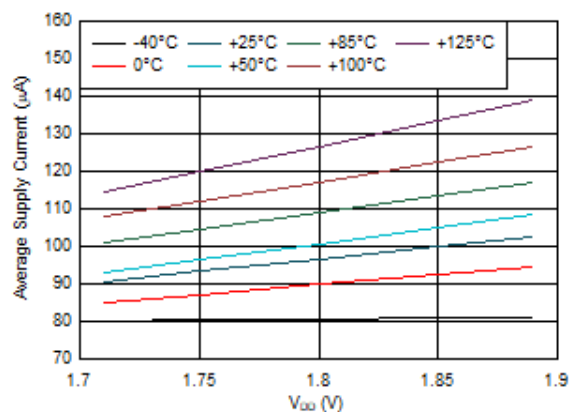
图 6-6. Supply Current vs. V_{DD} . Sensor R_P = 720\ \Omega , Scan Rate = 40 SPS, Sensor Frequency = 20 MHz.
