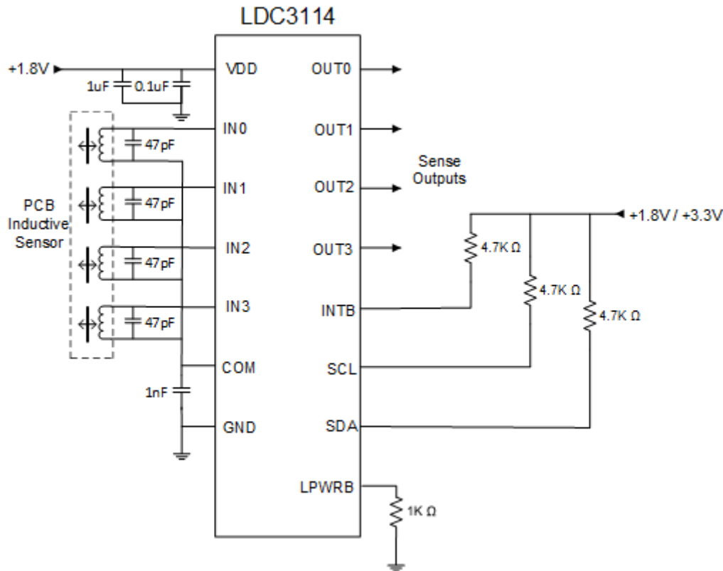
图 8-15. Application Schematic
