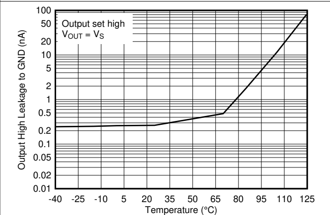
图 6-24. Output High Leakage Current vs. Temperature at 36V
