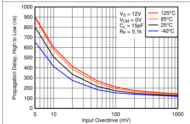
图 6-27. High to Low Propagation Delay vs. Input Overdrive Voltage, 12V
