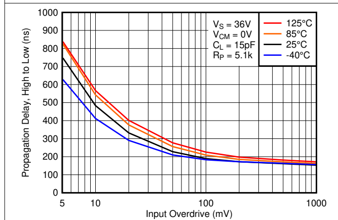
图 6-29. High to Low Propagation Delay vs. Input Overdrive Voltage, 36V
