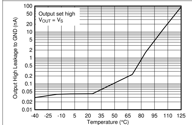
图 6-23. Output High Leakage Current vs. Temperature at 5V
