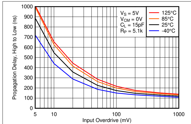
图 6-25. High to Low Propagation Delay vs. Input Overdrive Voltage, 5V
