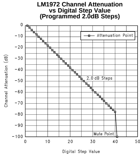
Figure 18. LM1972 2.0dB Attenuation Step Scheme
