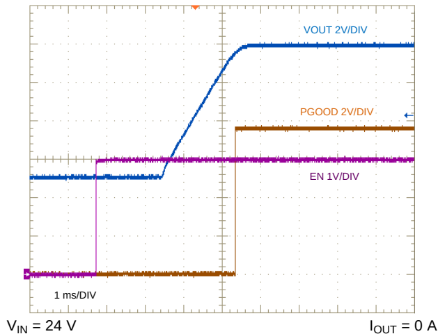
Figure 64. Pre-Biased Start-Up
