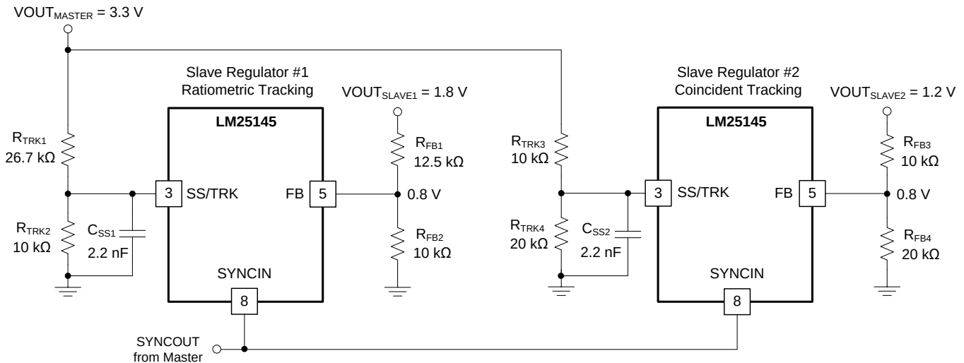
Figure 37. Tracking Implementation With Master, Ratiometric Slave, and Coincident Slave Rails
