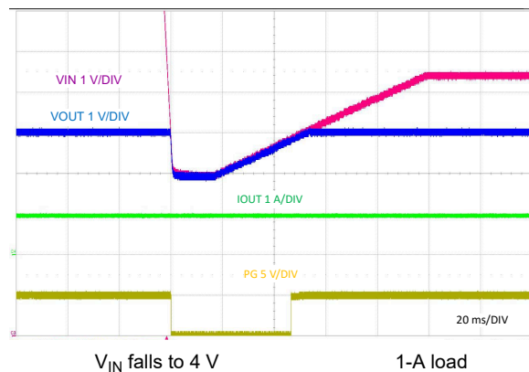
图 9-23. Cold-Crank Response to V_{IN} = 4 V
