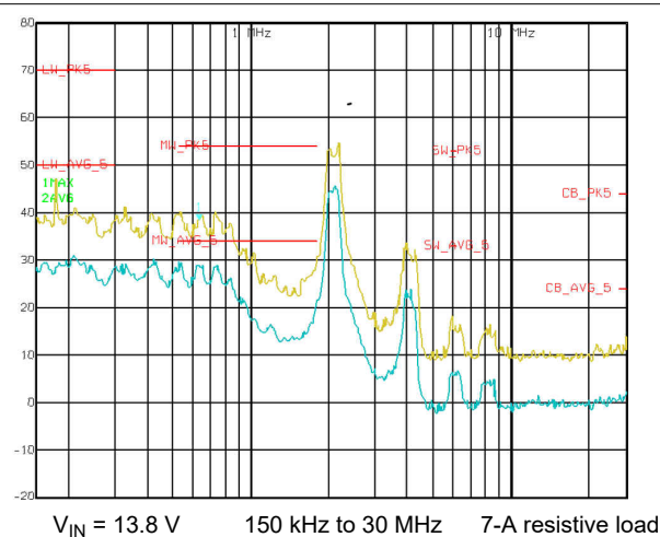
图 9-16. CISPR 25 Class 5 Conducted EMI
