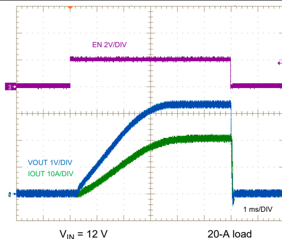
图 9-32. ENABLE ON and OFF Characteristic
