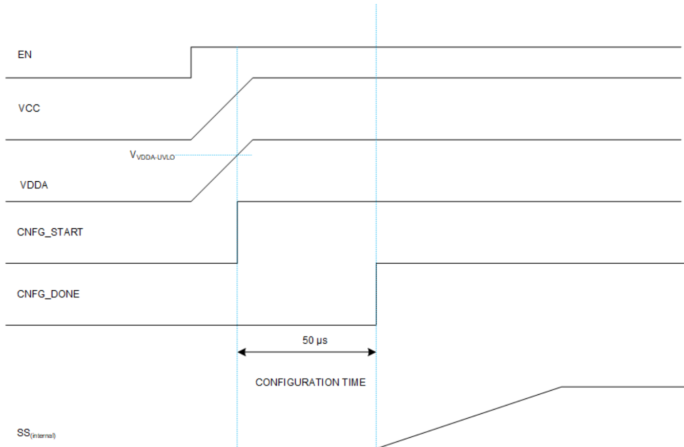
图 8-5. Configuration Timing
