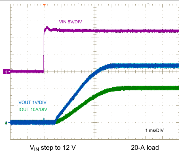
图 9-31. V_{IN} Start-Up Characteristic
