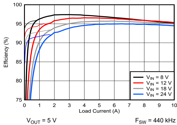
图 7-1. Efficiency vs. Load
