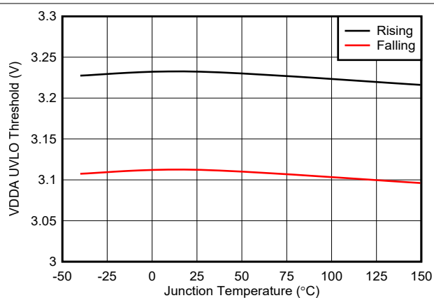
图 7-16. VDDA UVLO Thresholds vs. Temperature
