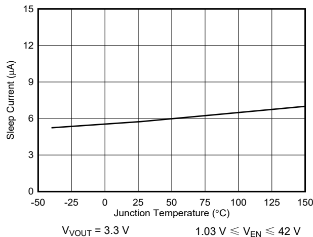
图 7-5. Sleep Current vs. Temperature
