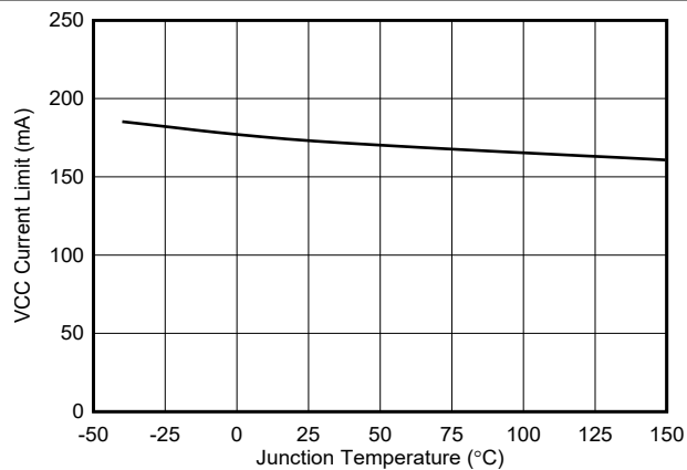
图 7-14. VCC Current Limit vs. Temperature
