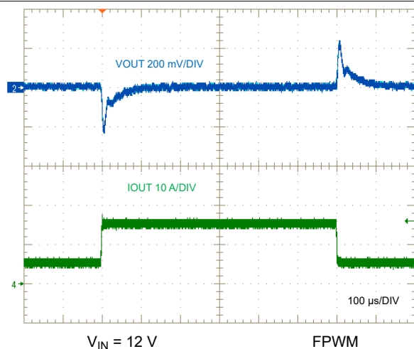
图 9-33. Load Transient, 5 A to 15 A
