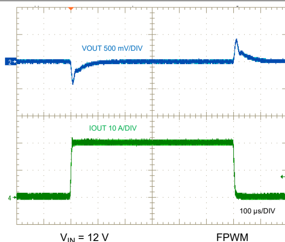
图 9-34. Load Transient, 0 A to 20 A
