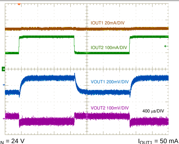
图 53. Output 2 Load Transient, 100 mA to 200 mA
