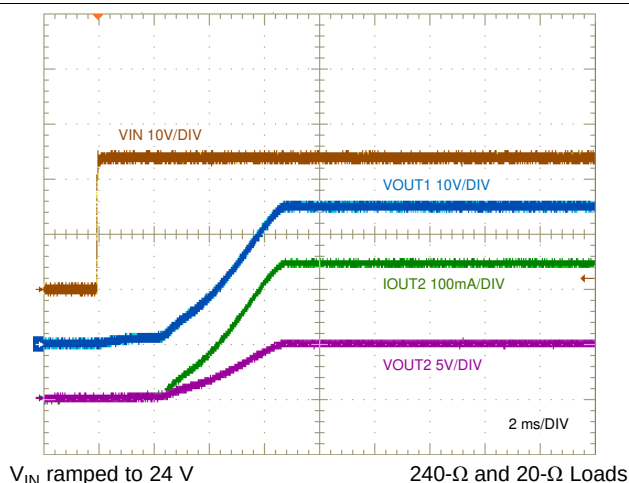
图 47. Start-Up Characteristic
