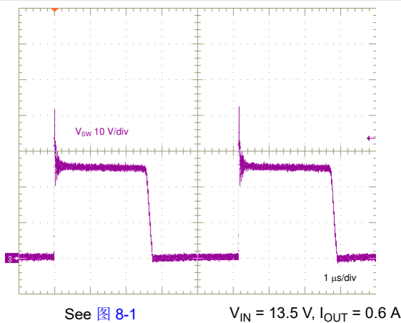
图 6-3. Switching Waveform in BCM
