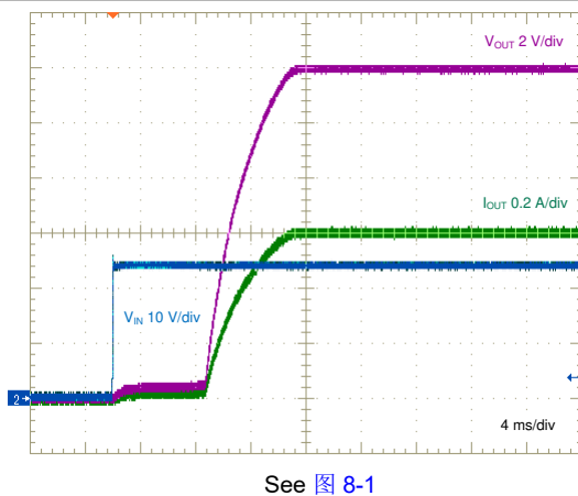
图 6-5. Start-up Characteristic
