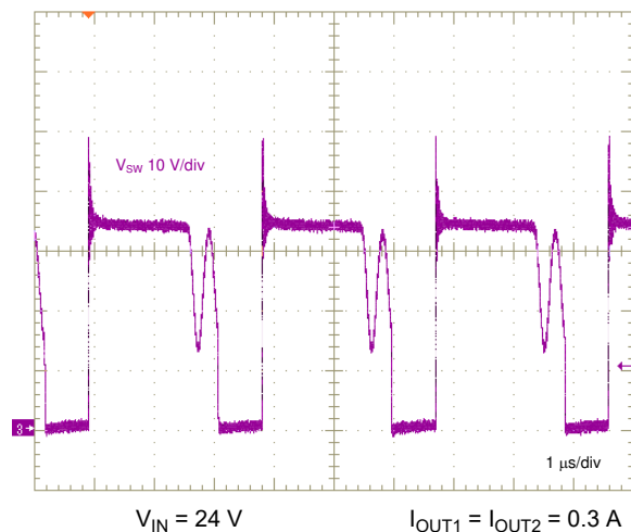
图 8-23. Switch Voltage, Medium Load
