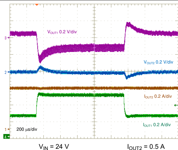
图 8-25. Positive Output Load Transient, 0.25 A to 0.5 A
