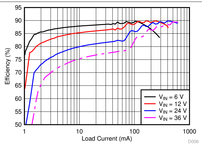
图 8-18. Efficiency (Log Scale)
