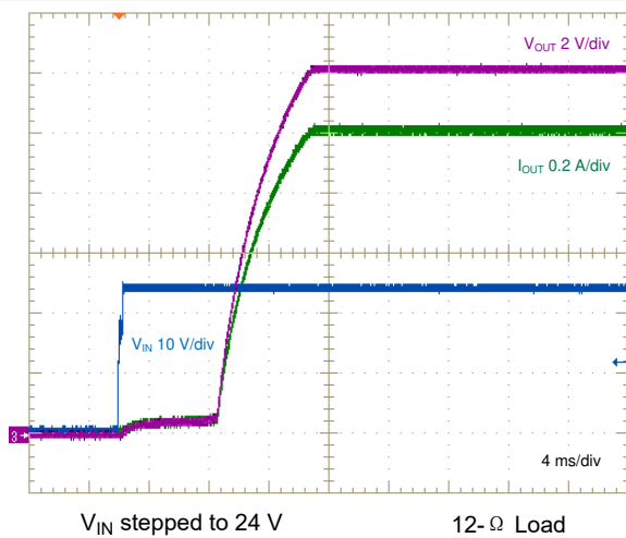
图 8-6. Start-up Characteristic
