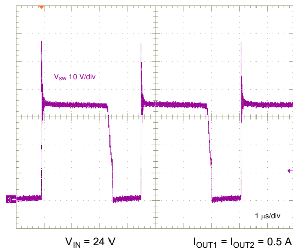
图 8-24. Switch Voltage, Full Load
