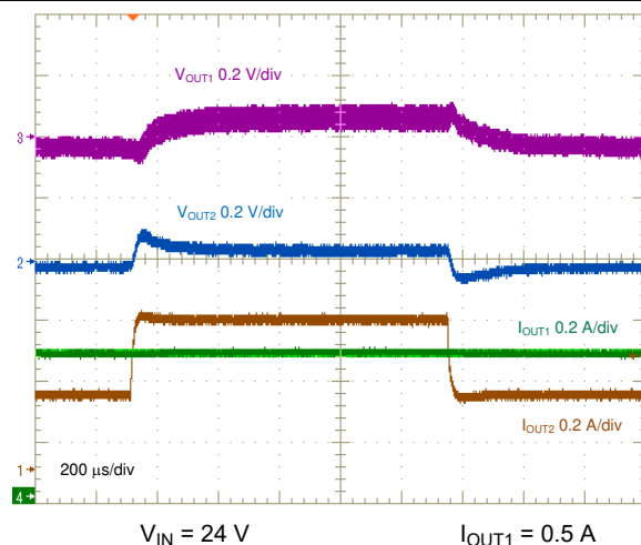
图 8-26. Negative Output Load Transient, 0.25 A to 0.5 A
