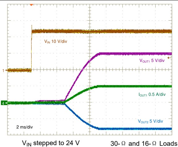
图 8-21. Start-Up Characteristic
