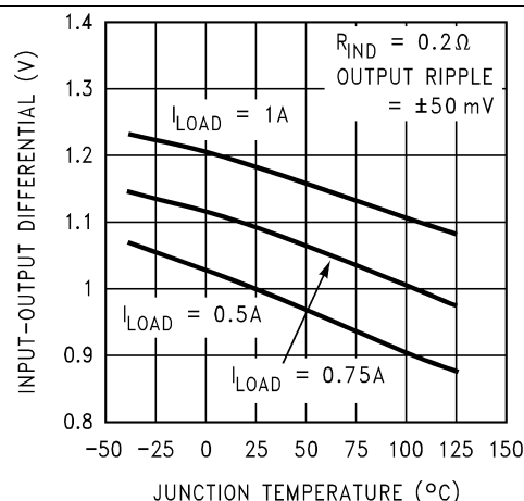
Figure 7. Dropout Voltage
