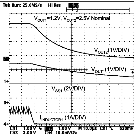
Figure 20. Thermal Shutdown
