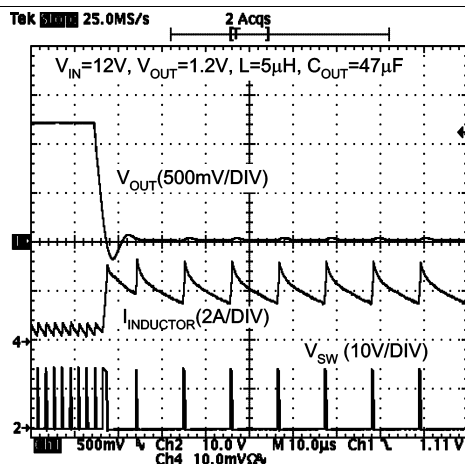
Figure 22. Short-Circuit Triggering
