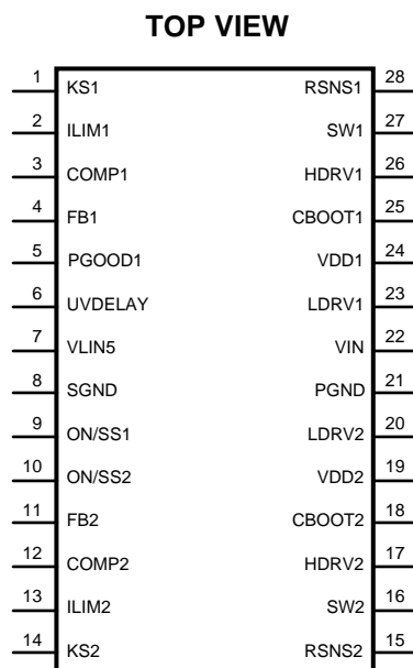
Figure 1. 28-Lead TSSOP
