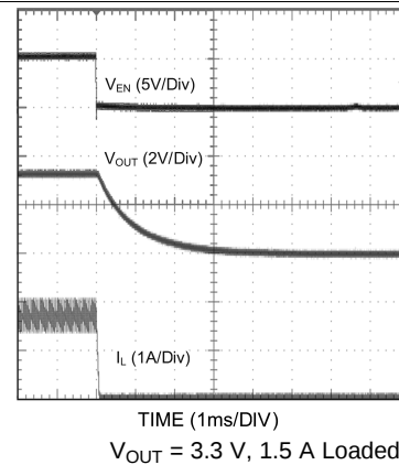
Figure 15. Shutdown Transient
