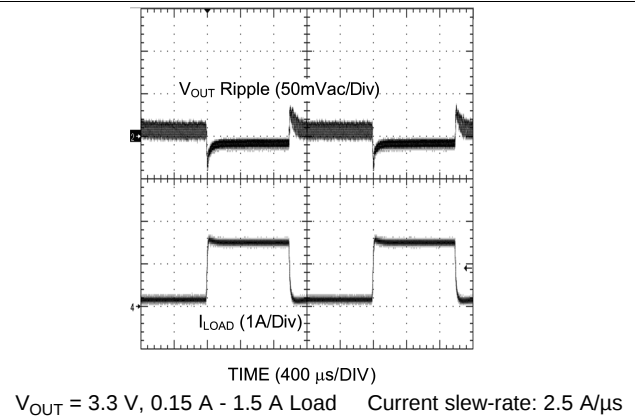
Figure 19. Load Transient
