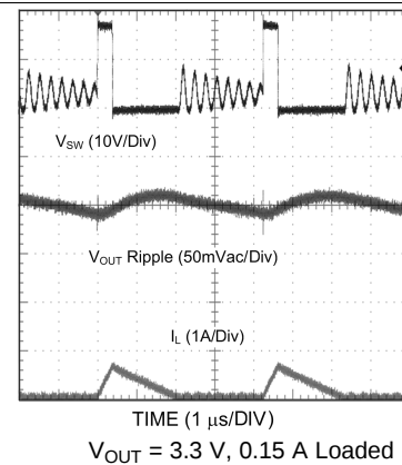
Figure 17. Discontinuous Mode Operation
