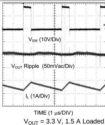
Figure 16. Continuous Mode Operation
