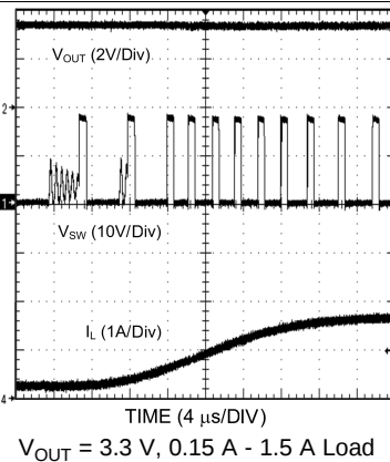
Figure 18. CCM to DCM Transition
