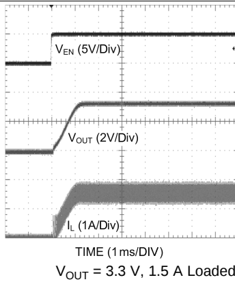
Figure 14. Enable Transient
