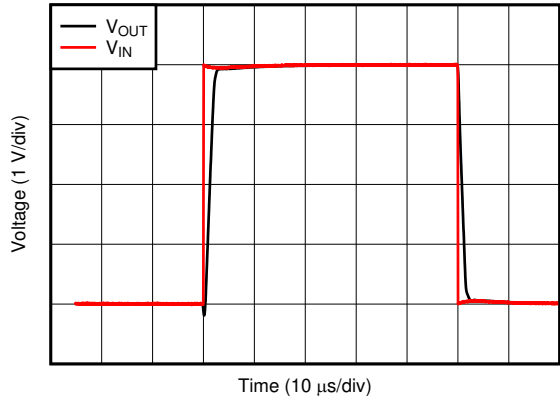
G = 1 V_{IN} = 4\text{V}_{PP} C_L = 10\text{pF} D030
