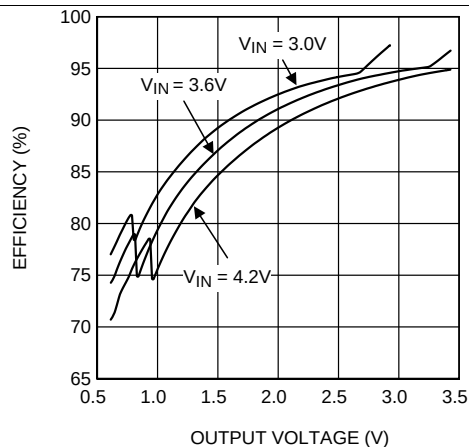
Figure 14. Efficiency vs Output Voltage
